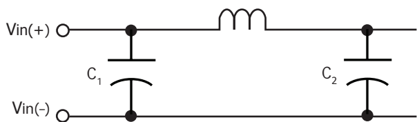
Figure E: Internal Input Filter Diagram (component values listed on page 3).
